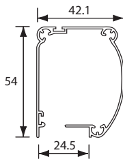
Cassette dimensions
