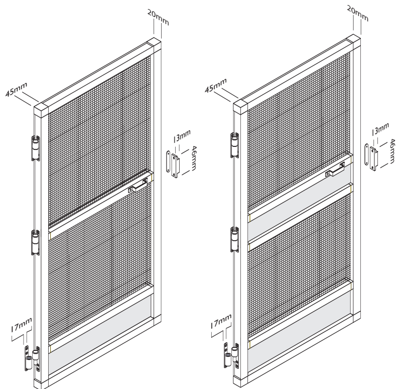
Commercial Door Screen with additional push plate
