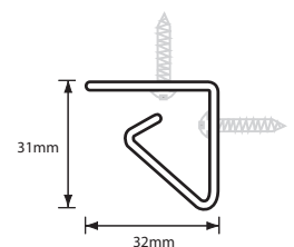
Profile and dimensions of hooked stainless steel track
